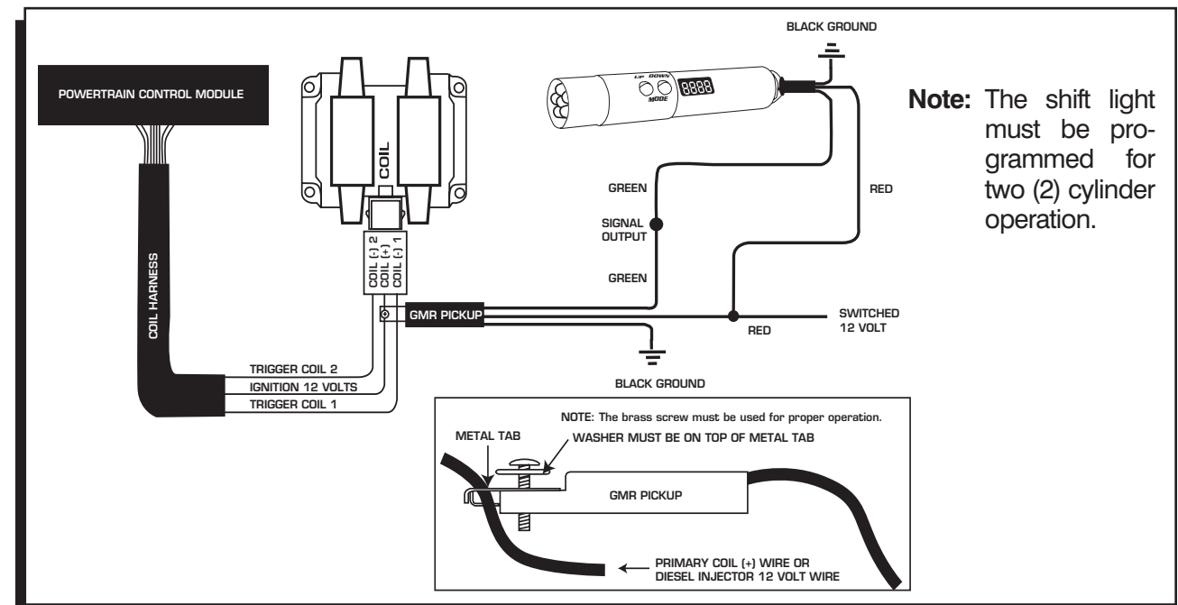
Figure 6 Installing to an Inductive Coil Pack.
